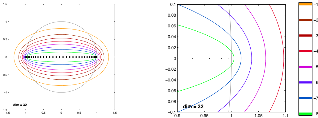
Fig. 1. Pseudospectra of A := \text{tridiag}(32, \frac{1}{4}, 0, 1)
